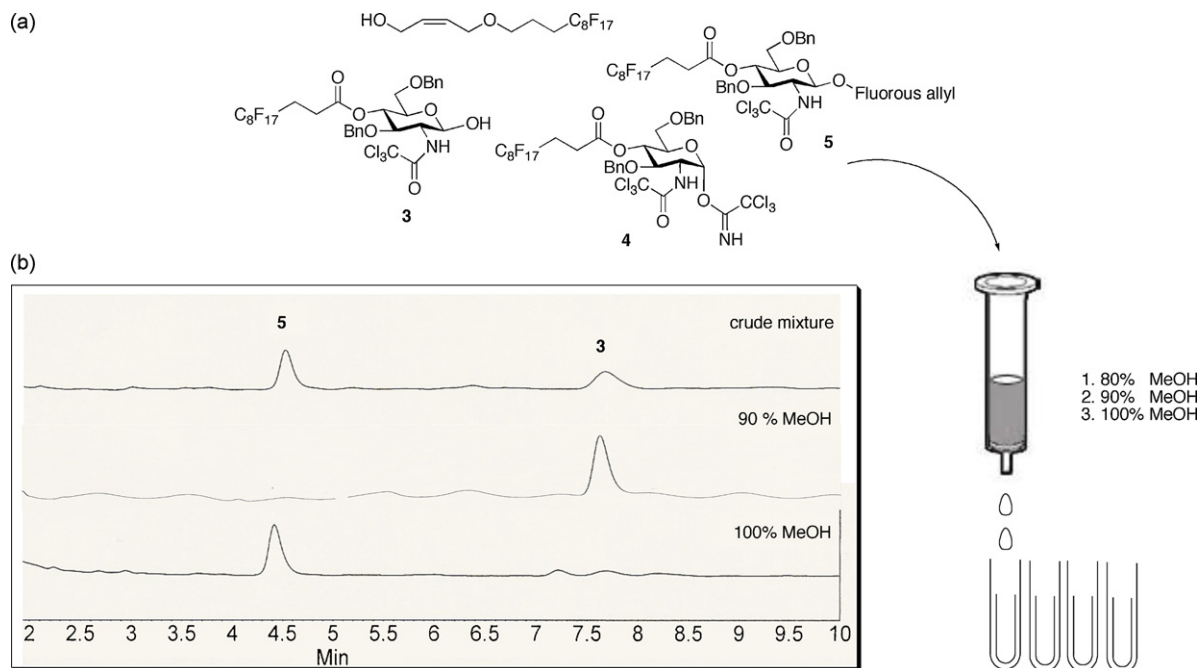
Fig. 2. (a) Selective elution of the multiple fluorous-tagged compounds using a FSPE cartridge and various elution conditions. (b) HPLC traces of the compounds eluted off the FSPE cartridge with 90% or 100% methanol elution. (HPLC conditions: 15% ethyl acetate/85% hexane, 1 ml/min flow rate, injection peak appeared at 1.5 min on a standard silica gel column.)
